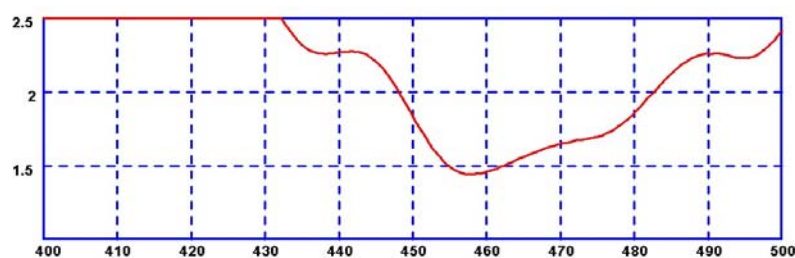
VSWR v Freq (MHz)
