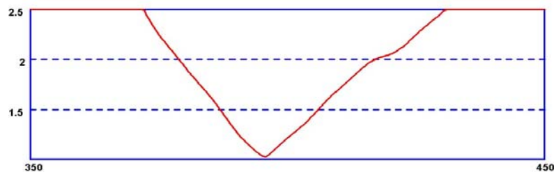
Typical VSWR v Freq (MHz)
