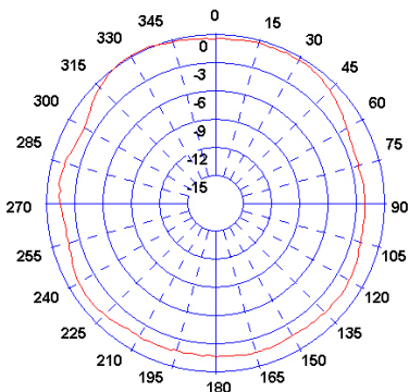
Typical Polar Plot @ 390 MHz
