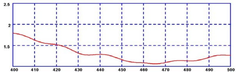
Typical VSWR v Frequency (Picture 460MHz)
