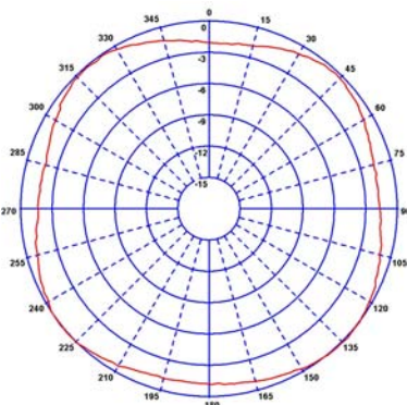
Typical Polar Plot (Picture 460MHz)
