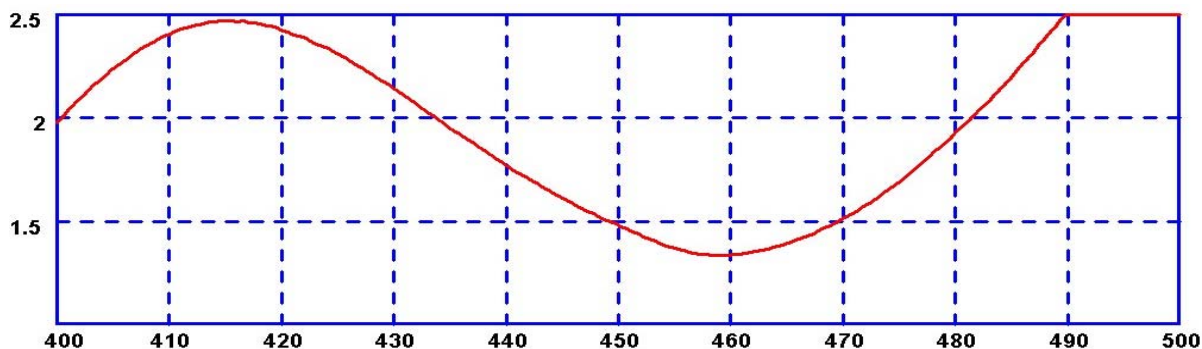
VSWR v Freq (MHz)
