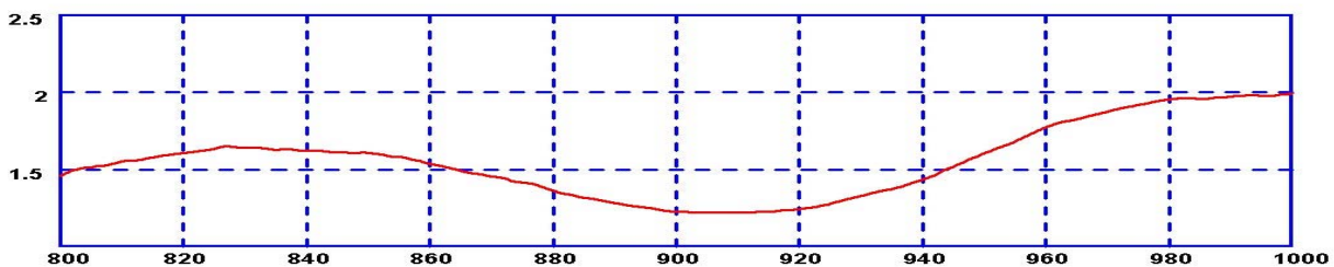
VSWR v Freq (MHz)
