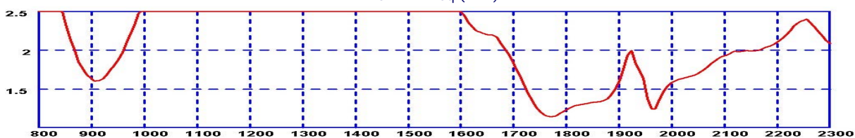
VSWR v Freq (MHz)
